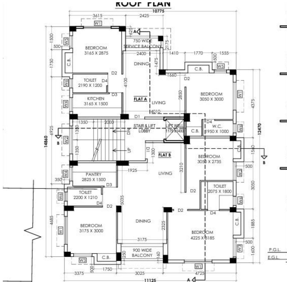
TYPICAL (1st, 2nd, 3rd & 4th) FLOOR PLAN
